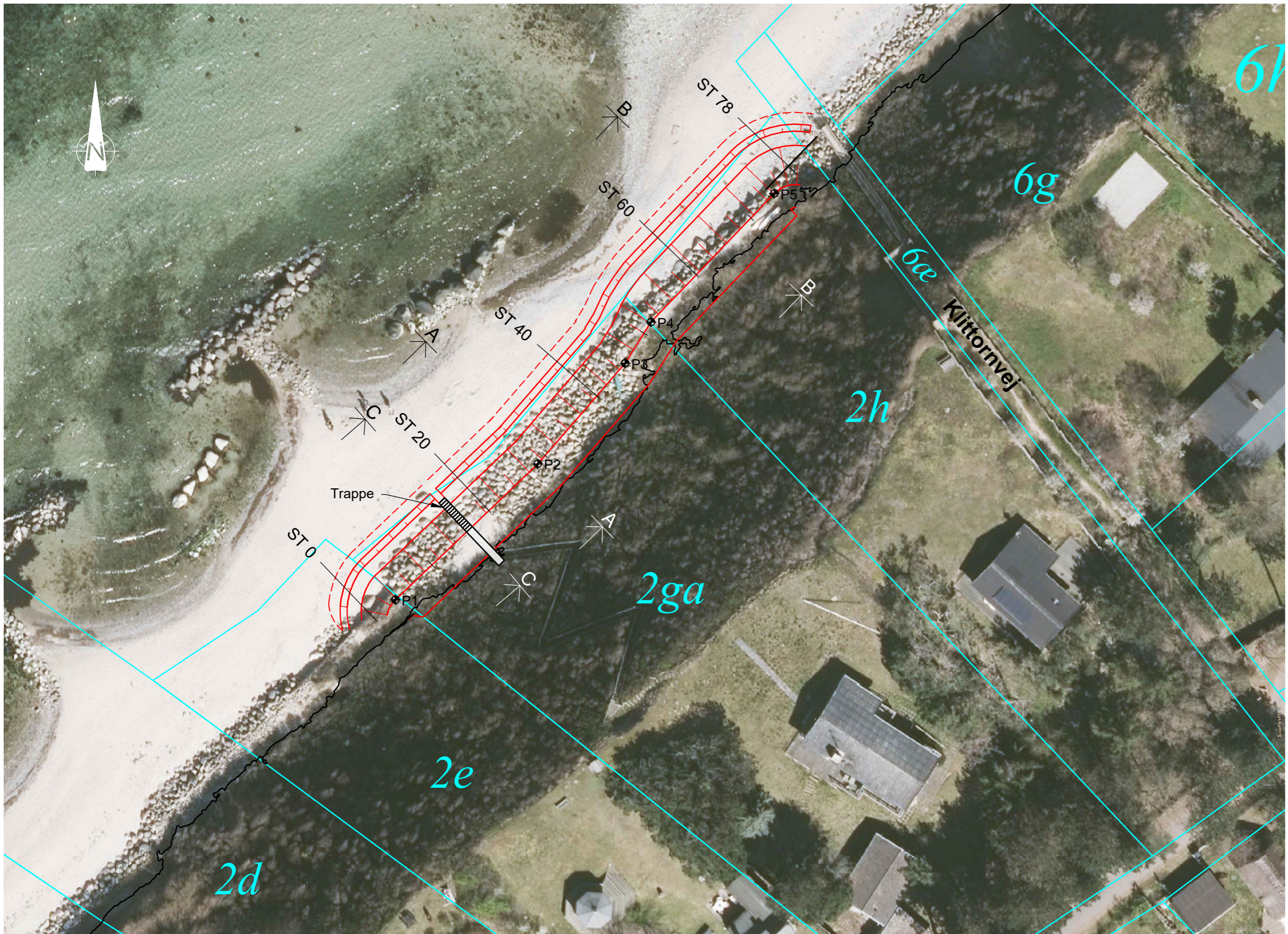
PLAN 1:500
